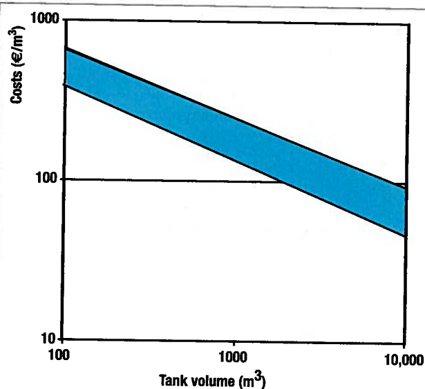
Figure 6. Free-standing insulated heat storage tank costs, including installation works
