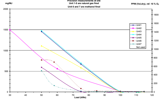
Figure 11. CO emission
