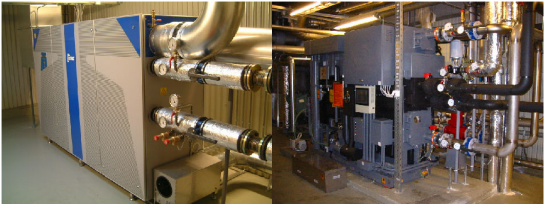
Figure 1. The Microturbine and Chiller Installation at Statoil, Stavanger
