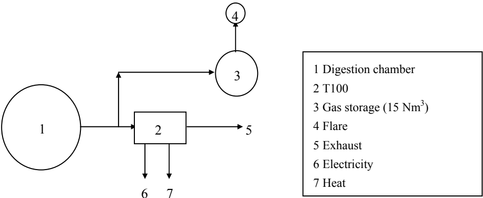
Figure 2. Schematic Installation of the Mariestad Site
