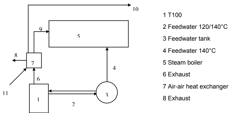
Figure 4. Schematic of the ICS Installation
