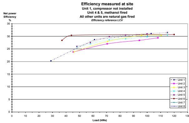
Figure 7. Power Efficiency Measurements on Site
