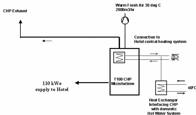
Figure 6. Schematic Installation of the SAS Radisson Site
