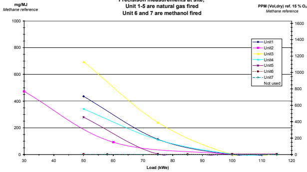
Figure 10. UHC emission
