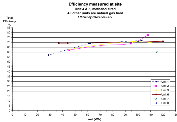
Figure 8. Electric Efficiency Measured at 7 Sites
