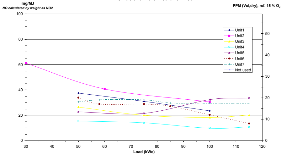
Figure 9. NO x emission
