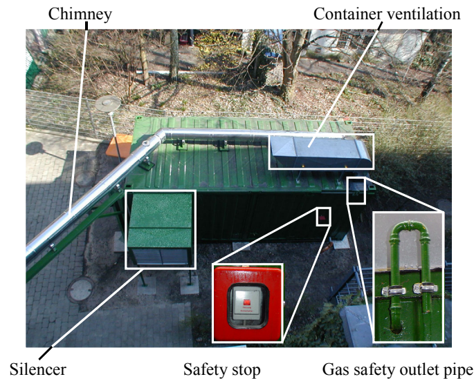
Figure 3. The Microturbine housing in a container at Hamburg
